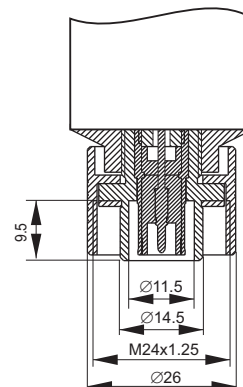
AD-26/CW Connector detail
