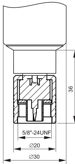
AD-25/CW-3512-S (connector detail)
