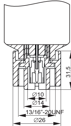
AD-25/CW-3512-S (connector detail)
