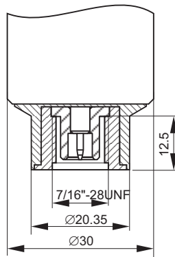
AD-25/CW-3512-H (connector detail)
