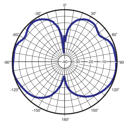
Rad. Pattern E-plane Frequency: 400 MHz
