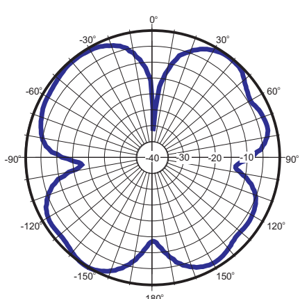
Rad. Pattern E-plane Frequency: 1000 MHz
