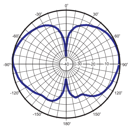
Rad. Pattern E-plane Frequency: 1400 MHz
