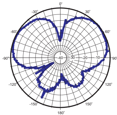
Rad. Pattern E-plane Frequency: 2500 MHz
