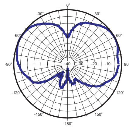
Rad. Pattern E-plane Frequency: 2200 MHz
