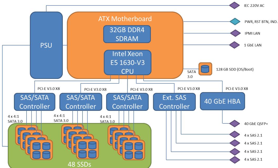
Figure 1: Functional block diagram of SP4000C
