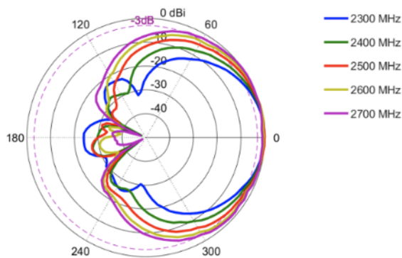
Azimuth: 2300 – 2700 MHz
