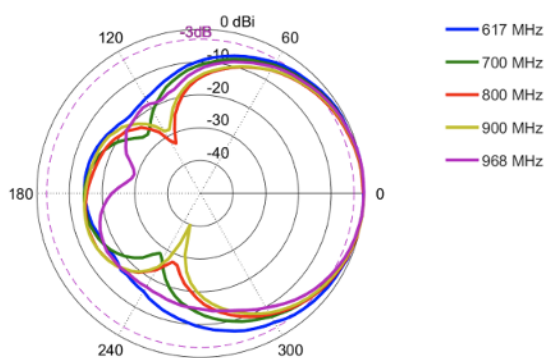
Azimuth: 617 - 968 MHz
