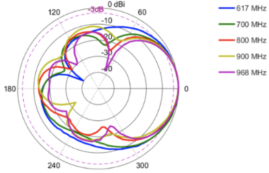
Elevation: 617 – 968 MHz
