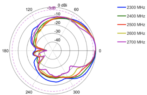
Elevation: 2300 – 2700 MHz
